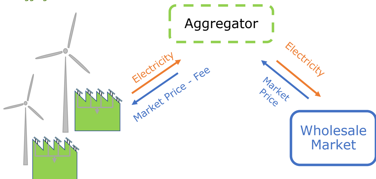
Aggregation model
