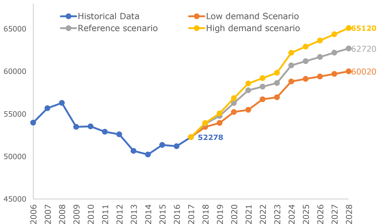
Forecast of total annual demand for electricity (GWh), [2006-2028]
